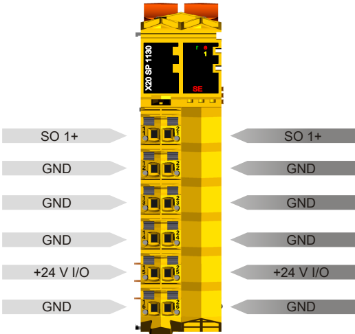
Figure 27: X20SP1130 - Pinout
