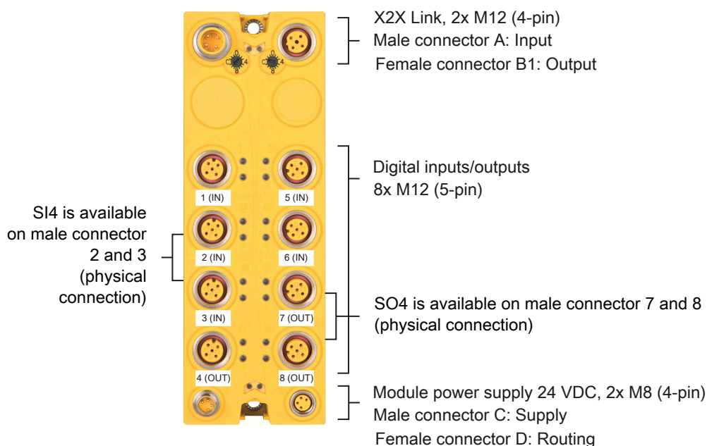
Figure 56: X67SC4122.L12 - Connection elements
