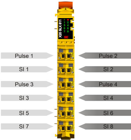
Figure 25: X20SLX811 - Pinout
