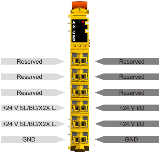
Figure 51: X20SL8101 - Pinout of the integrated power supply unit
