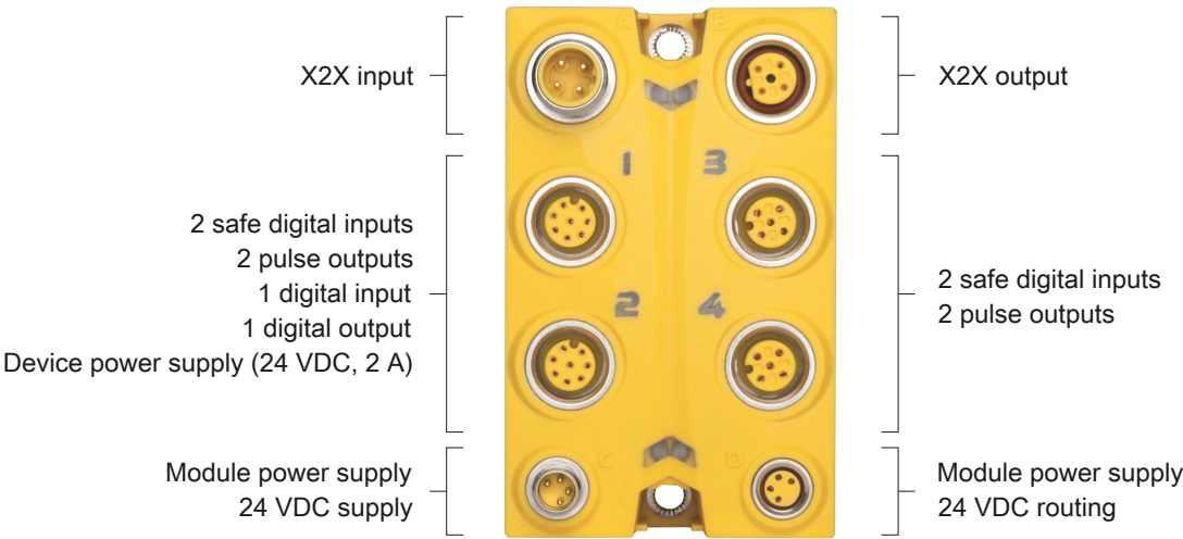
Figure 55: X67SI8103 - Connection elements
