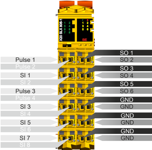
Figure 16: X20SLX806-1 - Pinout
