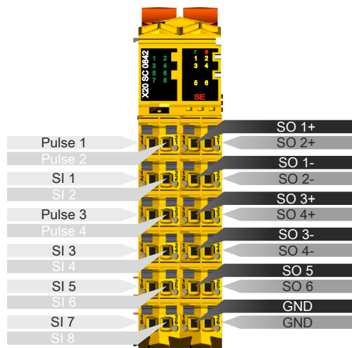
Figure 13: X20SC0842 - Pinout
