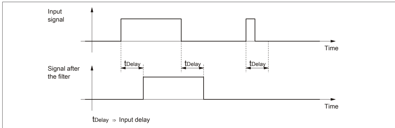
Figure 92: Input filter
