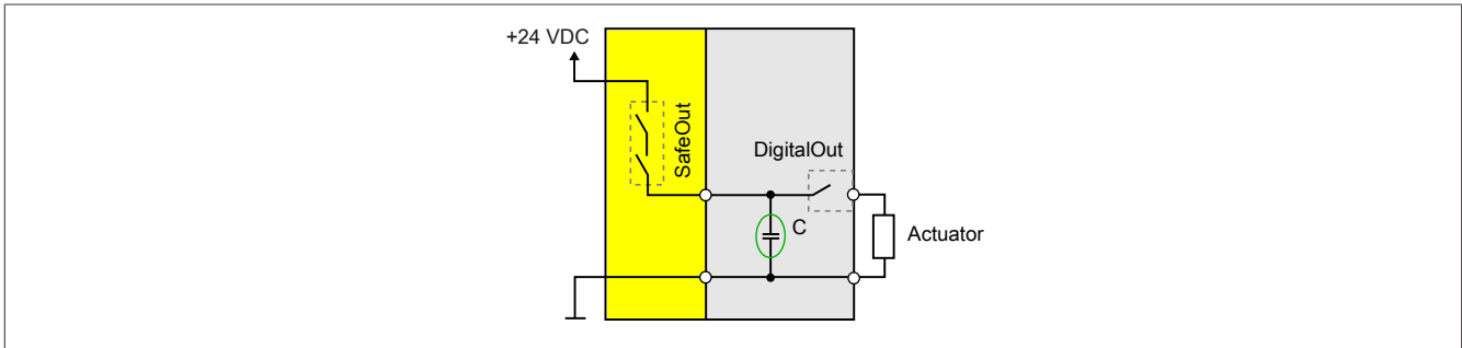
Figure 85: Functionality with internal energy storage
