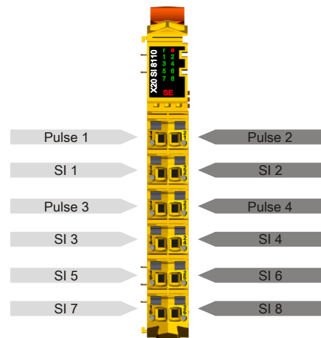
Figure 4: X20SI8110 - Pinout
