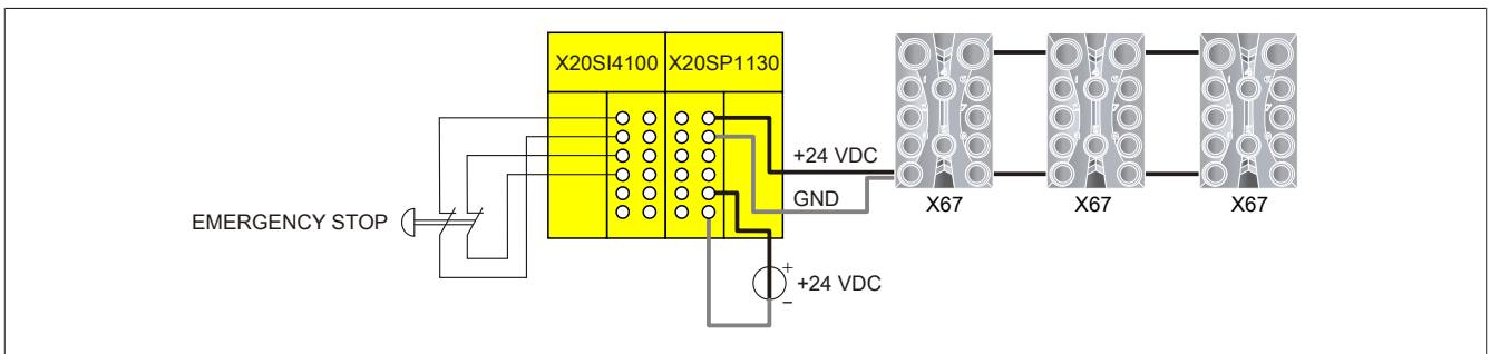
Figure 87: Circuit example with power supply module X20SP1130 and X67
