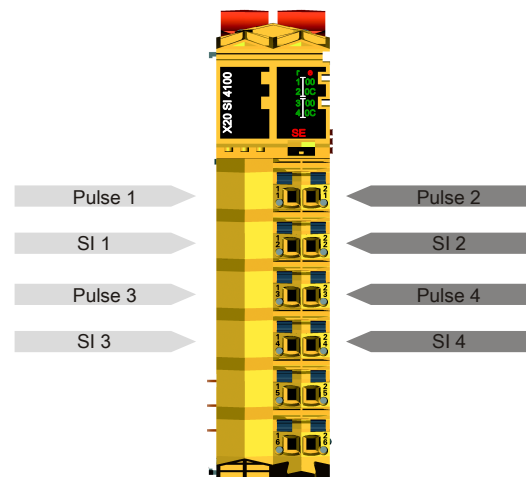
Figure 2: X20SI4100 - Pinout
