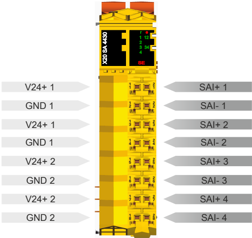
Figure 28: X20SA4430 - Pinout
