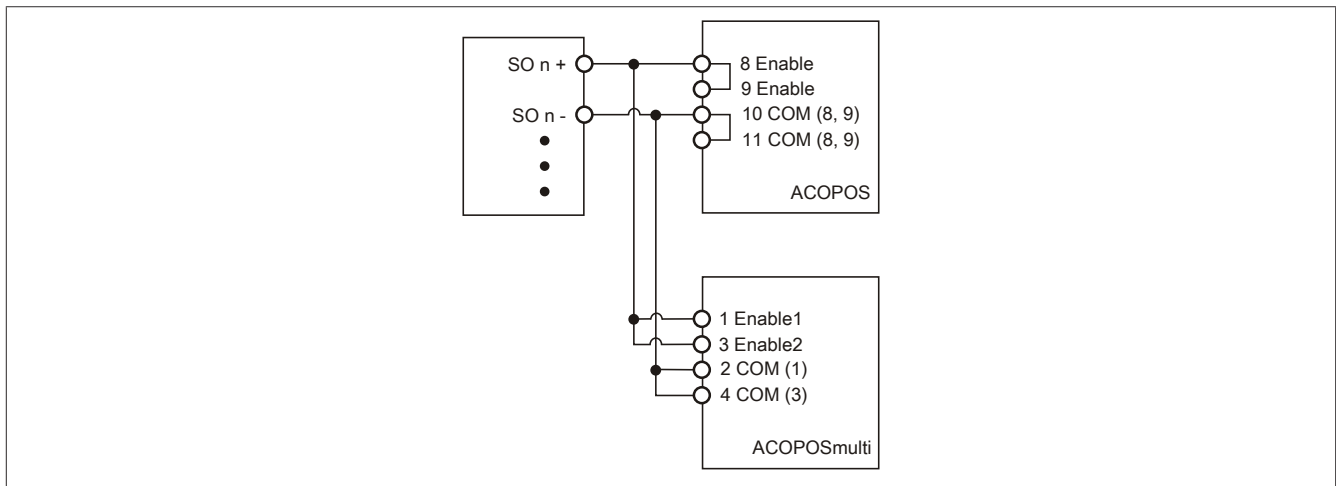
Figure 75: Connecting ACOPOS/ACOPOSmulti
