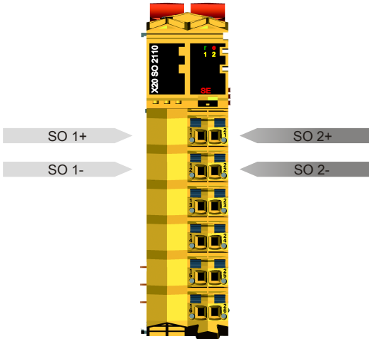
Figure 7: X20SO21x0 - Pinout
