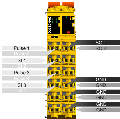
Figure 11: X20SC0402 - Pinout
