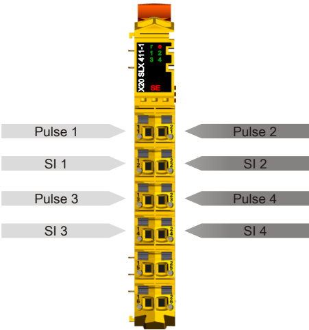
Figure 18: X20SLX411-1 - Pinout
