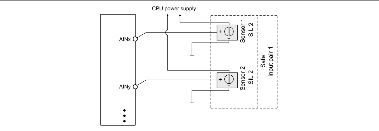
Figure 69: 3-wire connections, 2x SIL 2 - Voltage measurement
