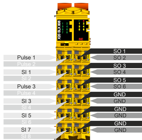
Figure 21: X20SLX806 - Pinout
