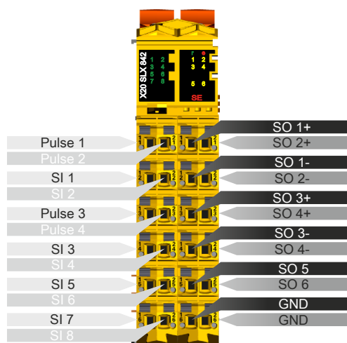
Figure 22: X20SLX842 - Pinout
