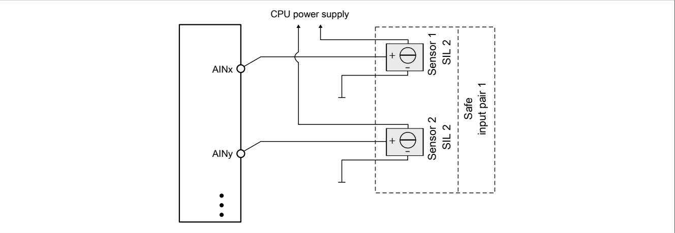
Figure 68: 3-wire connections, 2x SIL 2 - Current measurement
