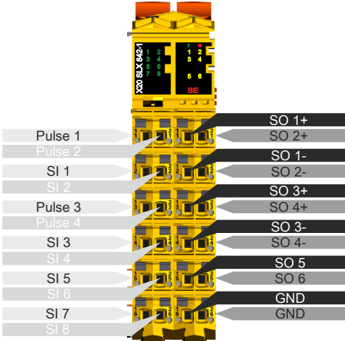
Figure 17: X20SLX842-1 - Pinout
