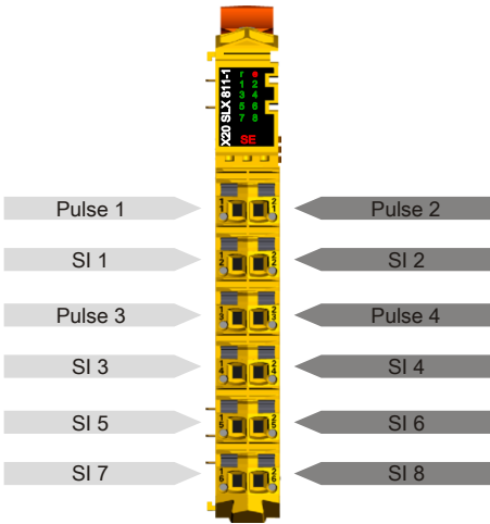
Figure 19: X20SLX811-1 - Pinout
