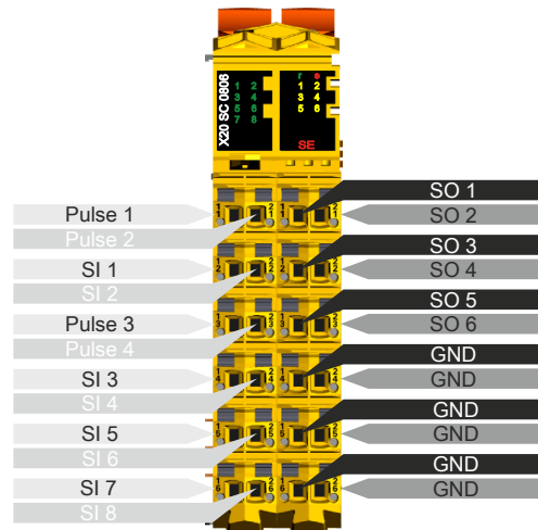
Figure 12: X20SC0806 - Pinout
