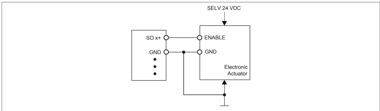
Figure 73: Connecting electronic actuators
