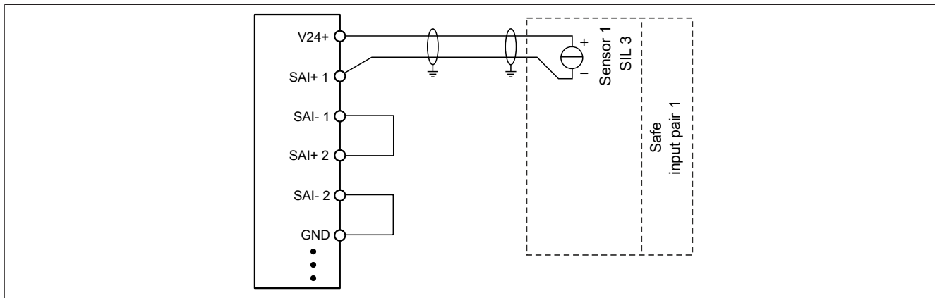
Figure 62: 2-wire connections, 1x SIL 3
