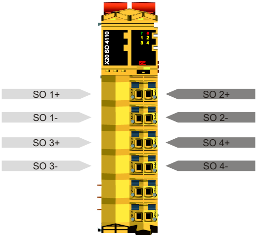
Figure 8: X20SO41x0 - Pinout
