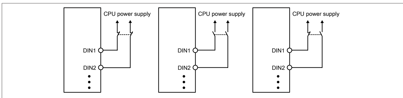
Figure 102: Connecting two-channel sensors with contacts
