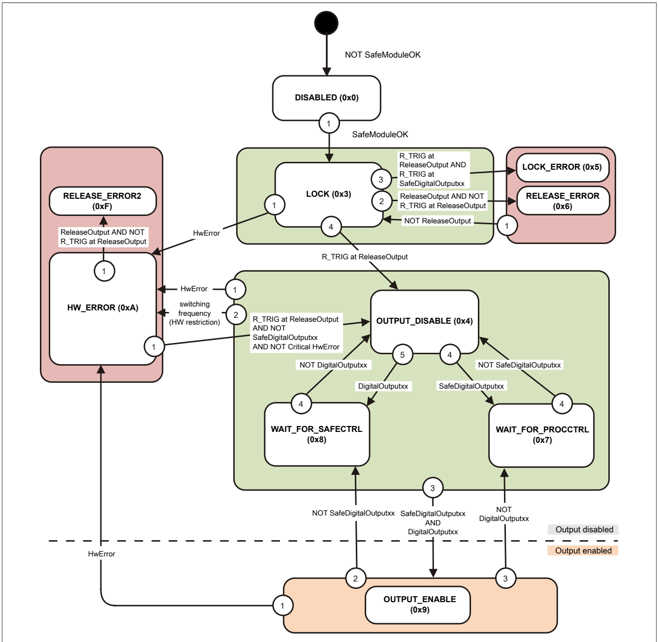
Figure 90: Error interlock - State diagram
