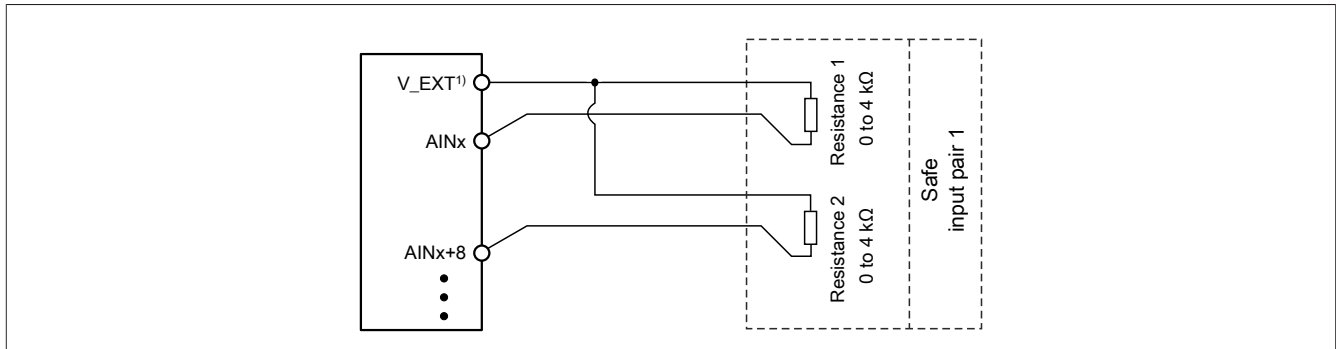
Figure 67: 2-wire connections, 2x SIL 2 - Resistance measurement
