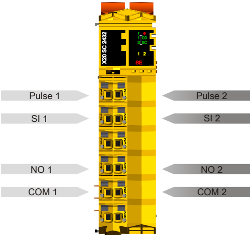
Figure 15: X20SC2432 - Pinout
