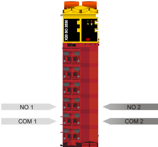
Figure 9: X20SO2530 - Pinout
