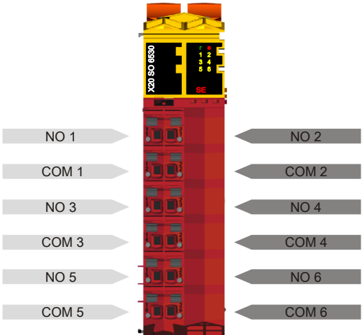
Figure 10: X20SO6530 - Pinout
