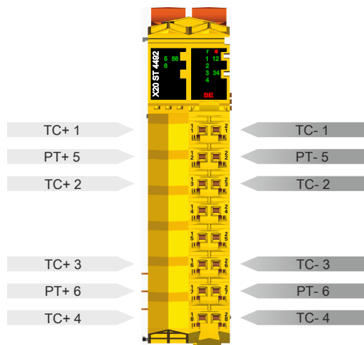
Figure 29: X20ST4492 - Pinout
