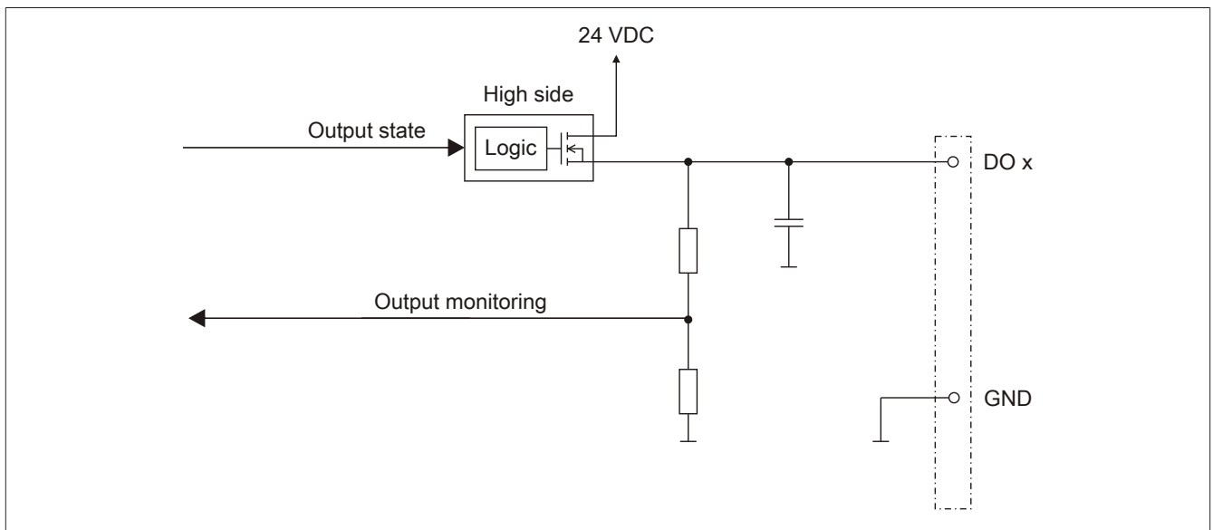
Figure 43: Output circuit diagram - Standard output without safety function
