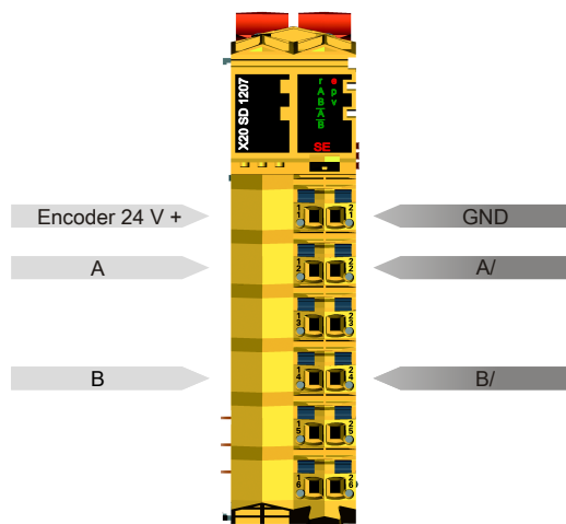
Figure 30: X20SD1207 - Pinout
