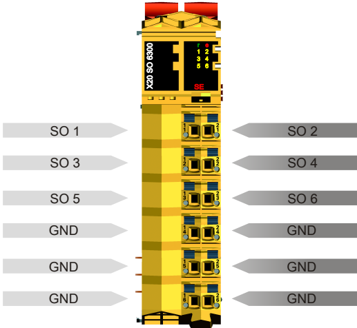
Figure 6: X20SO6300 - Pinout
