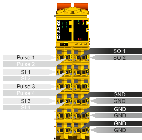
Figure 20: X20SLX402 - Pinout
