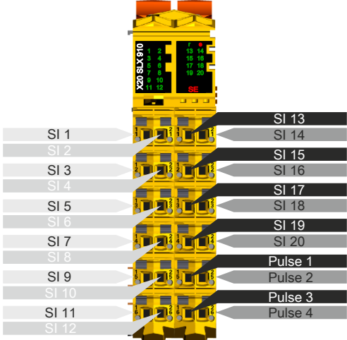
Figure 26: X20SLX910 - Pinout
