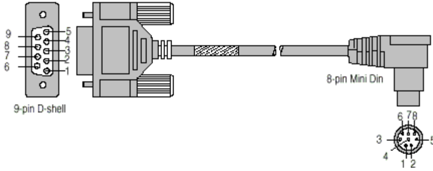
1761-CBL-PM02 Series B (or equivalent) Cable Wiring Diagram
