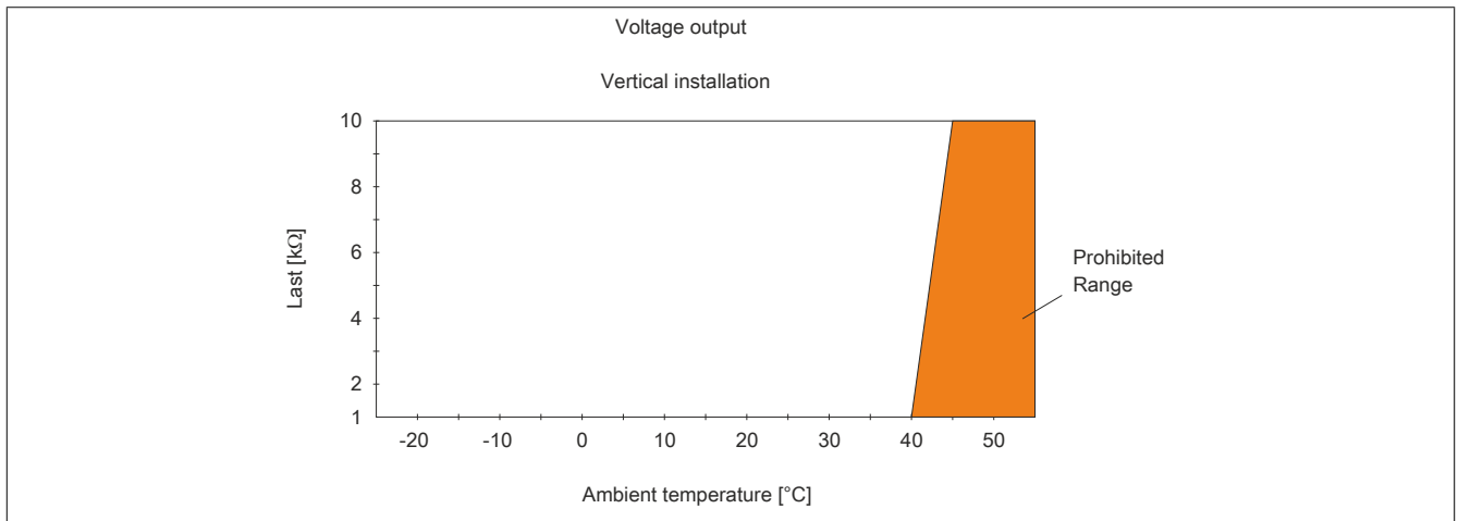
Figure 3: Derating the load with a voltage output and vertical mounting
