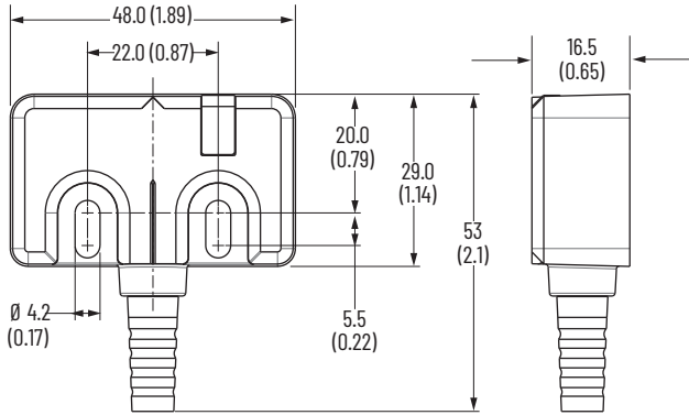
Figure 1 - Unit Dimensions [mm (in.)]
