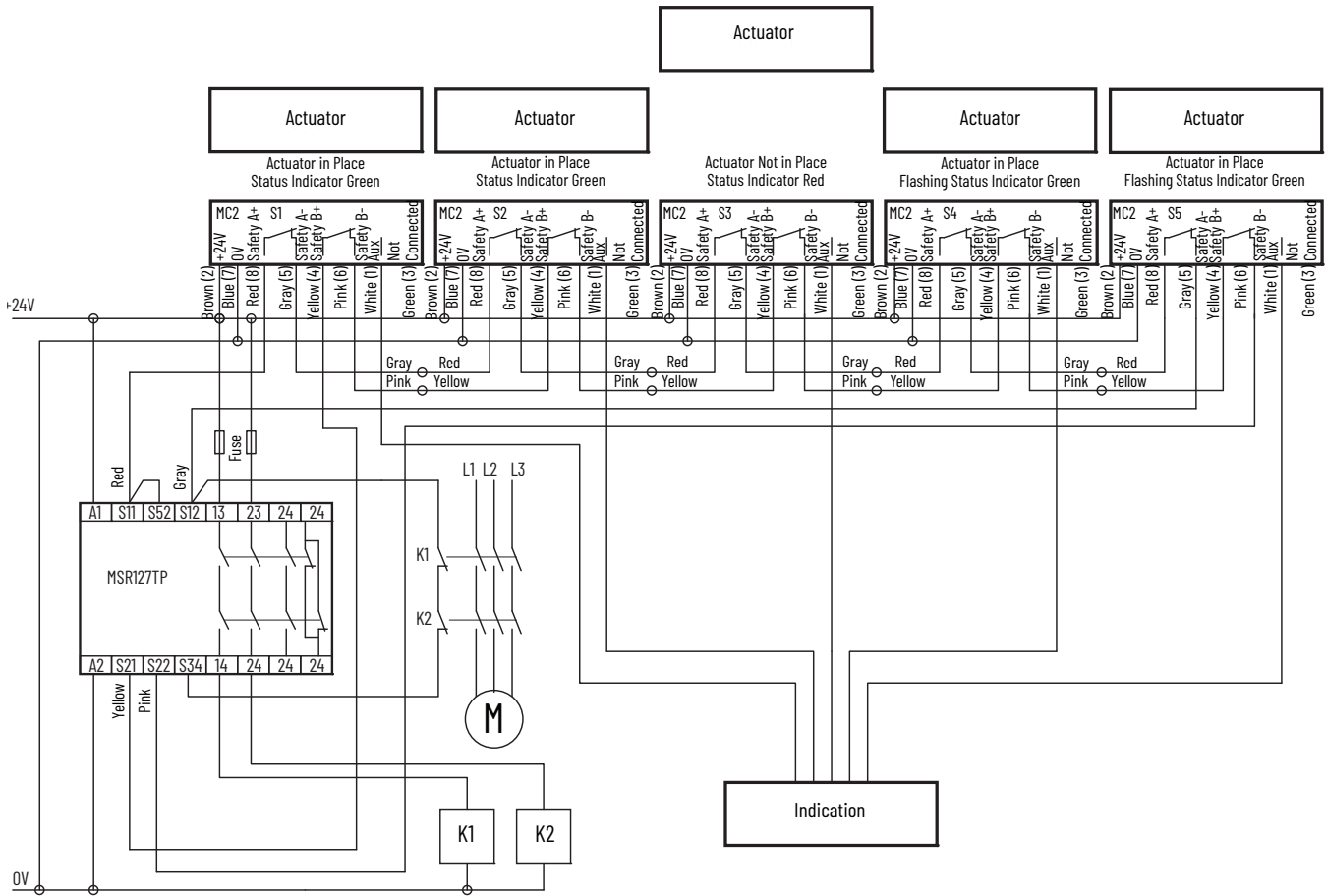
Figure 7 - Multiple Switches, Automatic Reset, Monitored Output MSRI27TP Safety Relay
