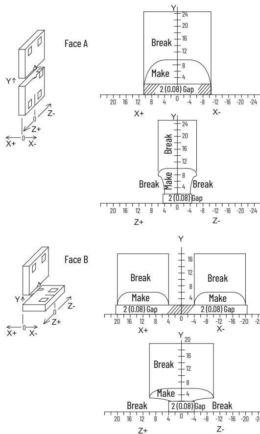
Figure 3 - Misalignment Curve [mm (in.)]
