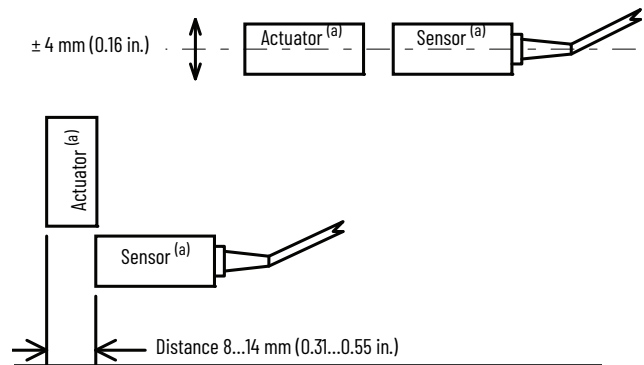
Figure 2 - Sensor Alignment
