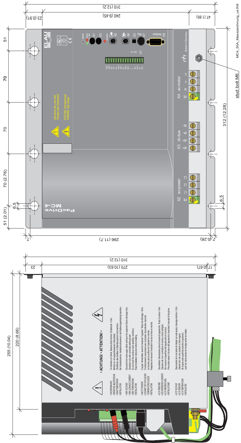
Fig. 6-6: Dimensions of the MC-4 / 50 A
