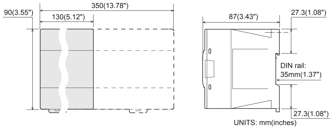
Figure 1.1: ENG ☞ Dimensioned unit FRE ☞ Dimensions GER ☞ Abmessungen ITL ☞ Dimensioni ESP ☞ Dimensiones
