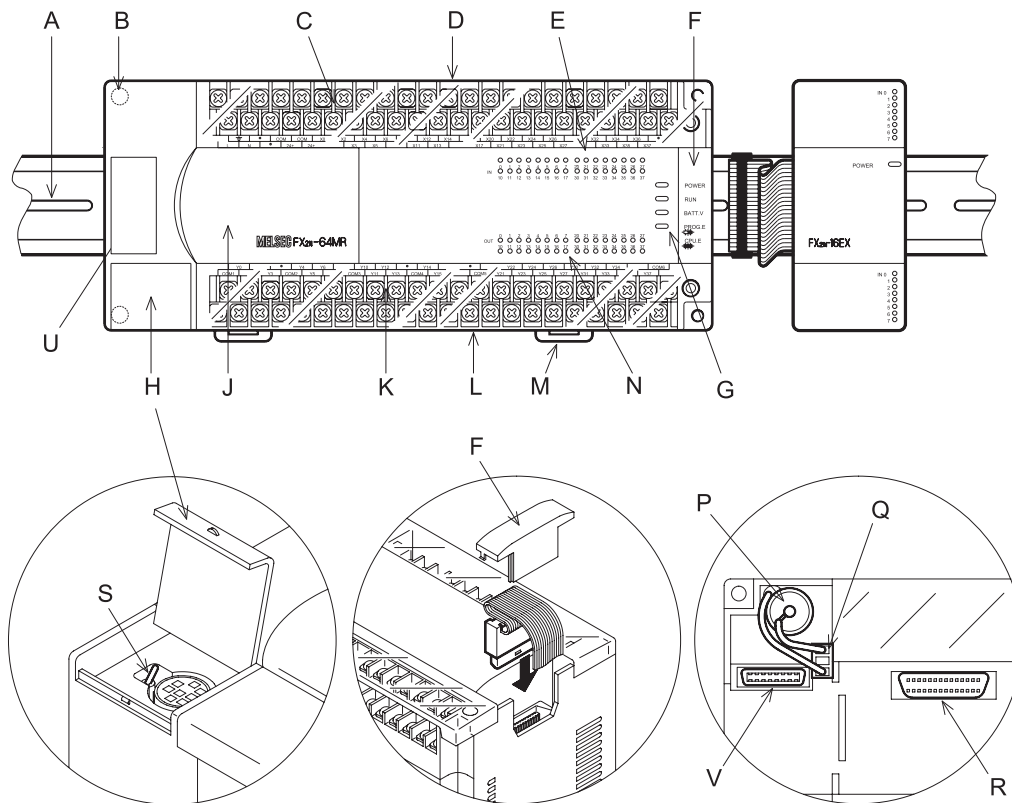
Figure 3.1: ENG Features of the FX2N PLC GER Beschreibung der FX2N-PS ESP Descripción de la FX2N-PLC FRE Description de l'API FX2N ITL Descrizione dell'FX2N-PLC
