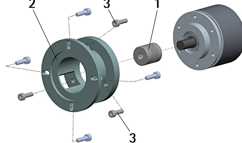
I58S, I58SK, I65 with mounting bell (order code PF4256)
